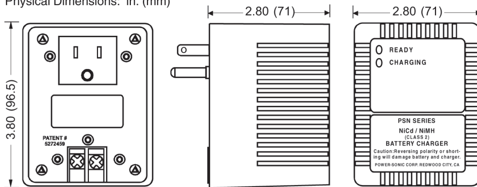
Physical Dimensions: in. (mm)
